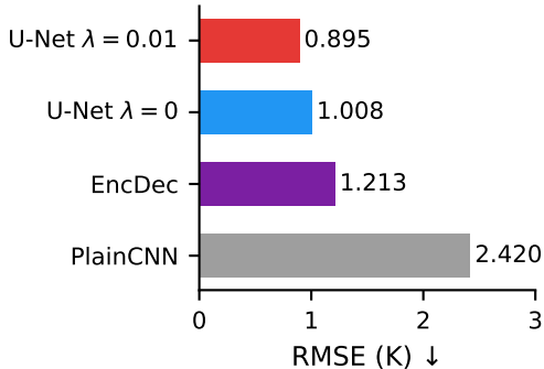
In-Distribution RMSE
